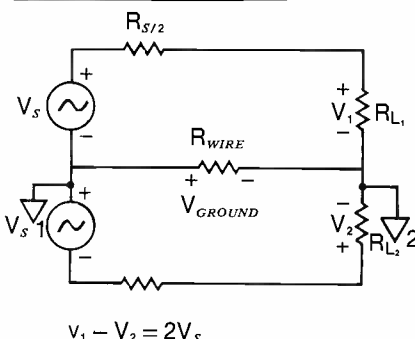
Figure 4. A balanced source where the amplitude error is eliminated.
